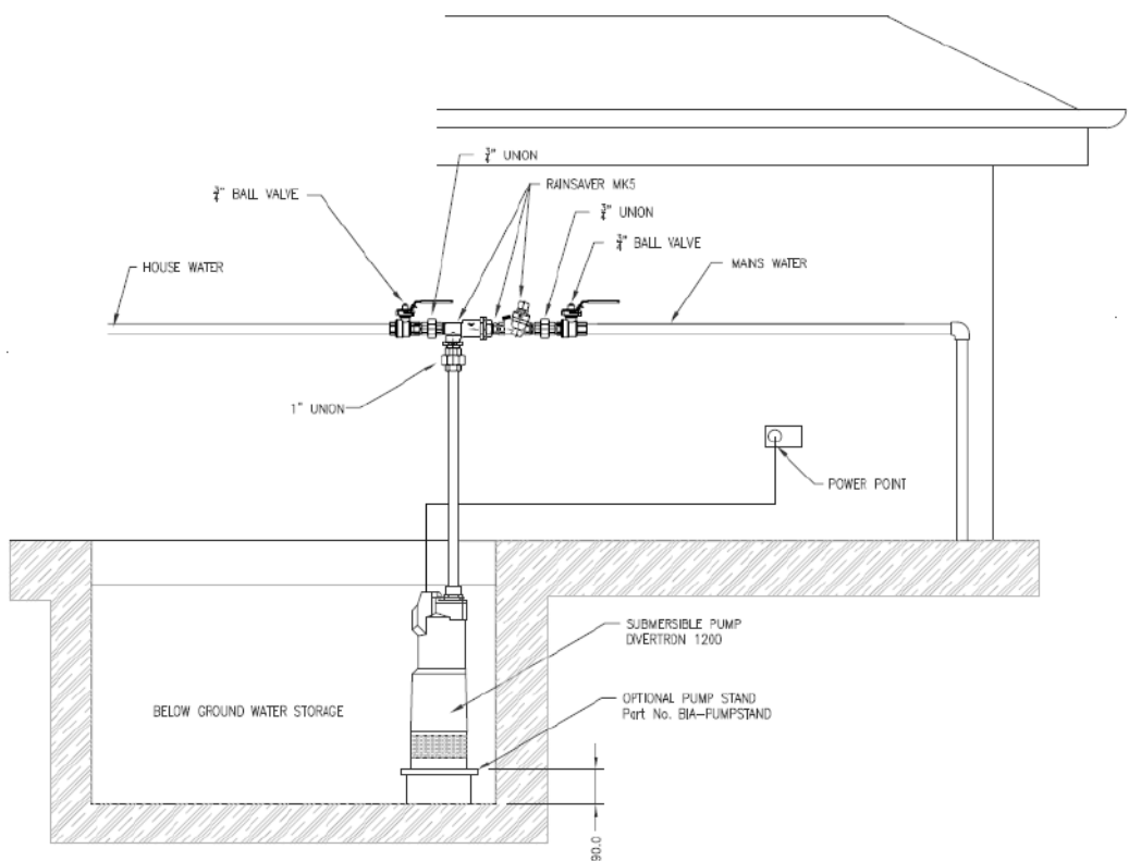
DAB DIVERTRON 1200 submersible pump with internal pump controller. RAINSAVERMK5 can be pipe mounted.
